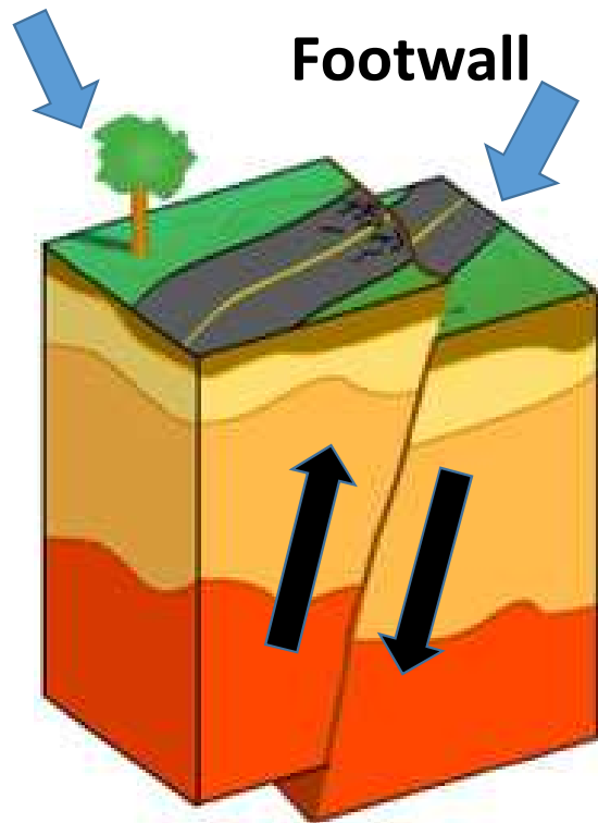
Reverse fault
