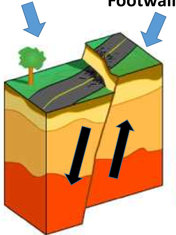
Normal fault
